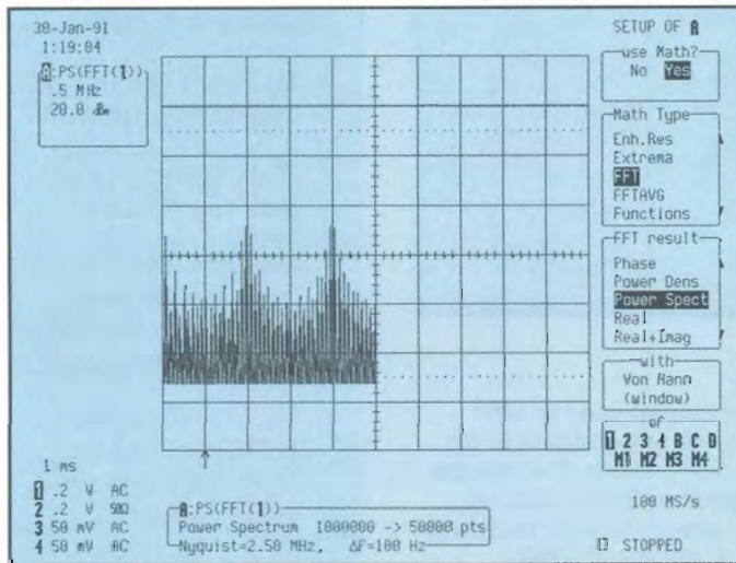
Without MWP option: The FFT processing of a 1 M point record length is limited to 50k; as a result the spectrum is limited to 2.5 MHz.
