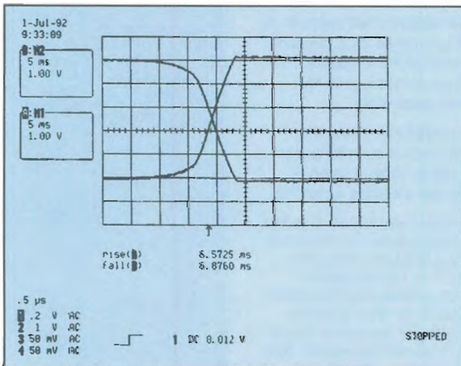
Figure 1: Switch-on transition of a dual output power supply (+5 V and -5 V). Symmetric behavior of the two voltages is often required. The automatic calculation of pulse parameters (rise and fall times in this case) simplify this test.
