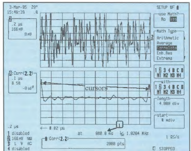
Figure 2. Autocorrelation reveals the underlying period of this waveform is 980.0 nanoseconds.
