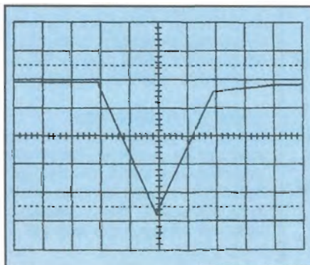
100 MS/sec digitizing of 5 nsec wide pulse
