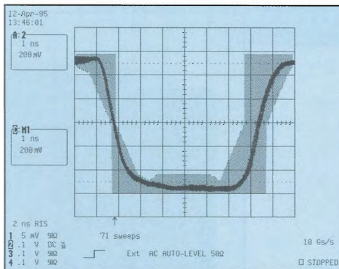
Figure 6: Mask test of a binary 1.
