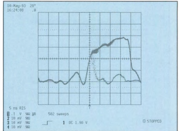
Figure 9. Flip-flop output exhibiting metastability.
