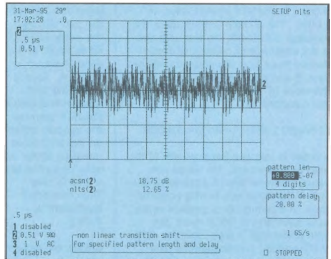
Figure 5. A waveform measurement with autocorrelated signal to noise and Non-Linear Transition Shift parameter measurements.
