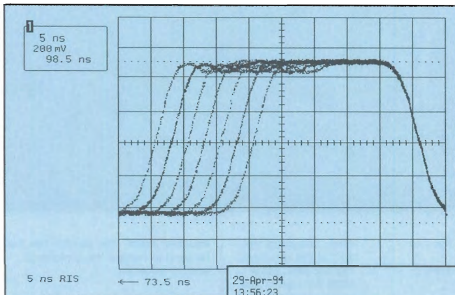
Figure 28. Leading edge jitter
