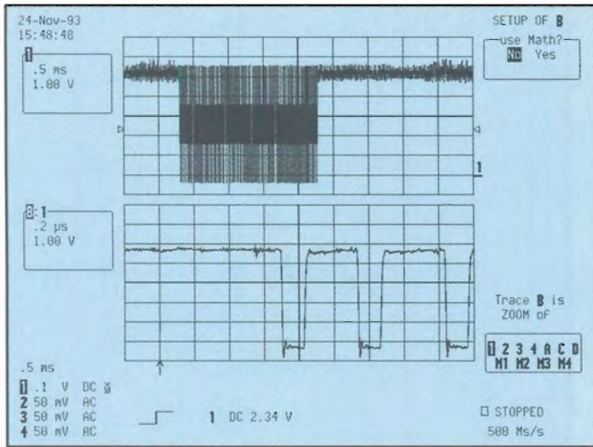
Figure 4. A burst of microprocessor communications activity. The expansion (lower trace) shows individual pulses in the train.
