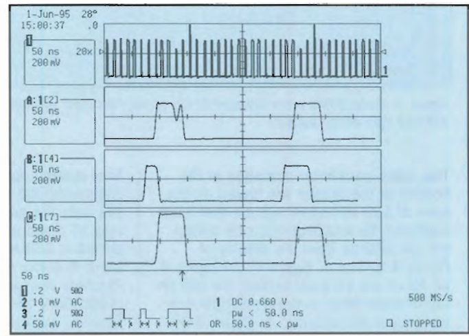
Figure 6. The compacted display of 20 events is on the top trace, on the other traces the zoomed detail of the 2nd, 4th and 7th event are shown.
