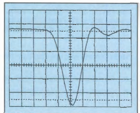
5 GS/sec RIS digitizing of 5 nsec wide pulse
