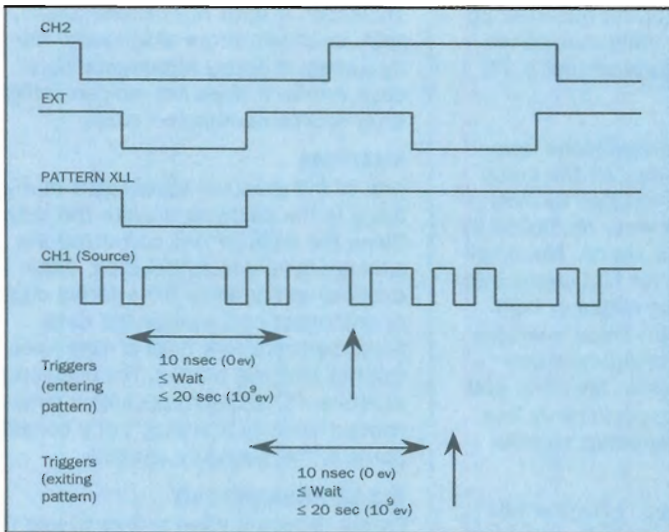
Figure 17: Timing diagram of the edge qualified trigger.
