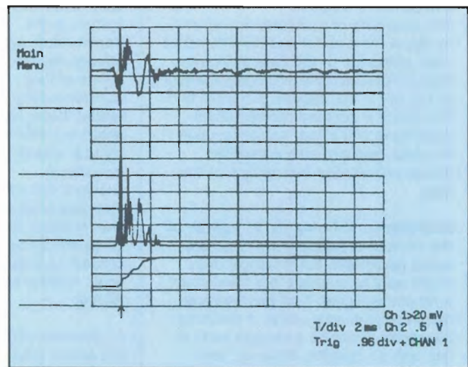
Figure 19: Current and voltage waveforms multiplied and integrated to display total energy.
