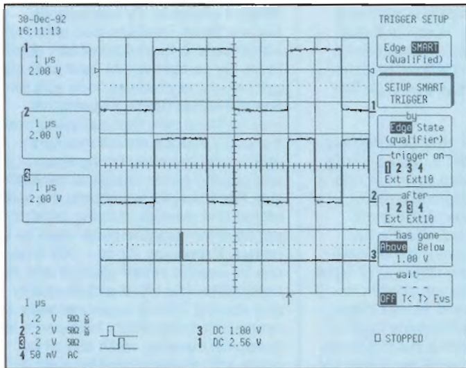
Figure 12: Logic Qualified (Pattern) Trigger: In this figure, acquisition is triggered on Channel 1's trigger conditions only after the signal on Channel 3 meets its own, independent set of trigger conditions. The trigger setup menu shows setup options, including delay (wait) by user-entered time or number of trigger events.
