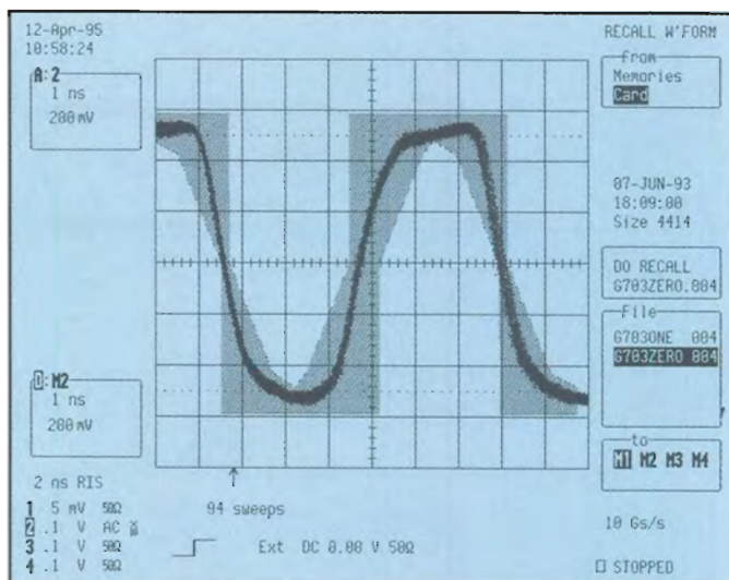
Figure 5: Mask test of a binary 0. Notice the jitter at the trailing edge of the pulse.
