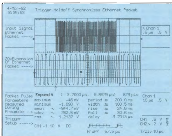
Figure 7: Trigger hold-off by time allows the above Ethernet signal to be displayed in its entirety as a stable trace despite repeated occurrences of valid trigger conditions. The 20:1 expansion in the lower trace and automatic pulse parameters characterize the packet's preamble.
