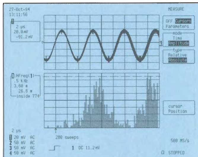
Figure 4: The top trace is a persistence display of a sinewave whose frequency is unstable. The histogram at the bottom shows that there are two components (two peaks) in the frequency distribution.
