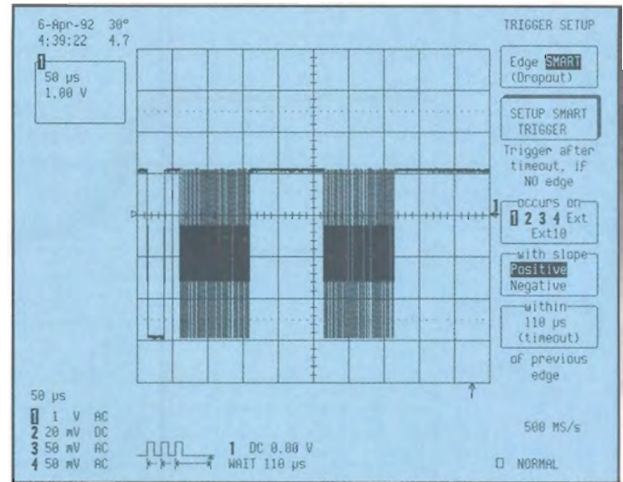
Figure 2: A DSO triggers on a "dropout". Note the scope is set to trigger if there is a gap of longer than 110 usec. Two data packets occur, but when a network collision causes the third packet to disappear the scope triggers.
