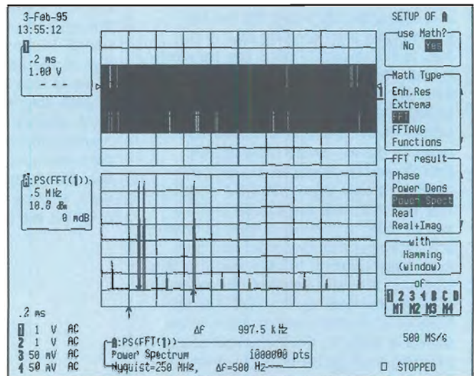
Figure 4b. An FFT of the same signal from Figure 4a with 1,000,000 points captured and analyzed. Now \Delta f is 500 Hz and the initial peak of Figure 4a is resolved into 2 peaks.
