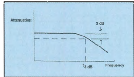
Attenuation occurs within the passband, not just at the cutoff (-3dB) frequency.
