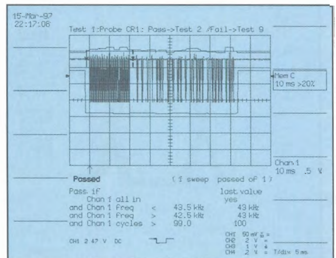
Figure 21: Testing an infra-red remote control unit. Note the simultaneous use of both parameters, such as frequency and number of cycles, and tolerance mask testing. Pass/Fail tests can incorporate up to 5 user-defined test conditions.
