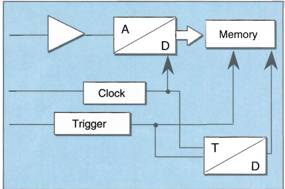
RIS digitizer block diagram
