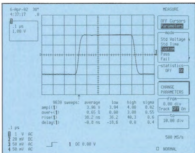
Figure 3: A DSO measures best and worst case shape of a data bit. In this case the maximum and minimum values are shown for pulse amplitude, positive overshoot, risetime and delay (timing jitter).
