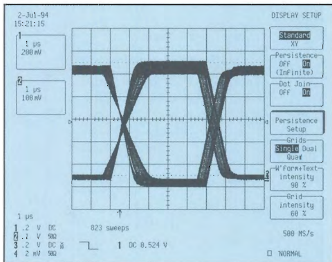
Persistence mode displays a user-selected number of sequential measurements.
