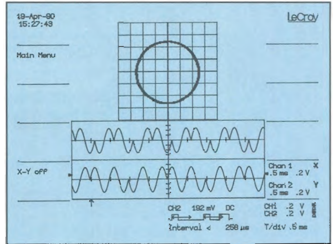
Figure 2. The phase trajectory of the I and Q components of a PSK signal.
