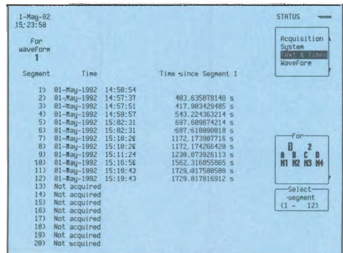
Figure 14. Time stamps associated with the collisions of Figure 13.
