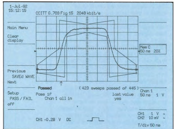
Figure 12. Automatic PASS/FAIL testing against a telecom template.
