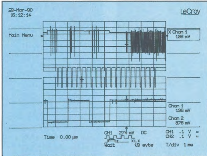
Figure 1. Interval trigger provides a stable trigger on a Phase Shift Keyed signal.
