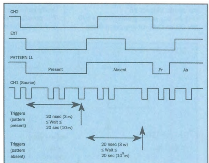
Figure 16: Timing diagram of the state-qualified trigger.
