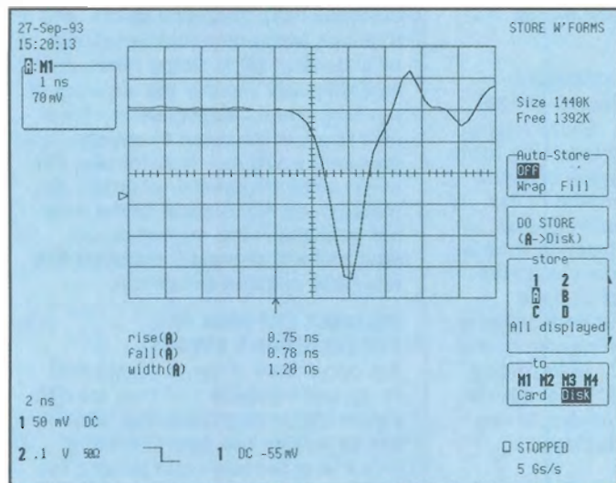
Figure 5: A typical 9354 display. Note the trigger level and source identified below the grid. The left-side and bottom arrows give a visual indicator of trigger level and time.
