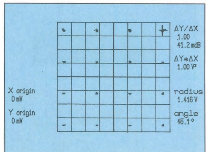
Figure 10. Constellation display of a 16-QAM signal.
