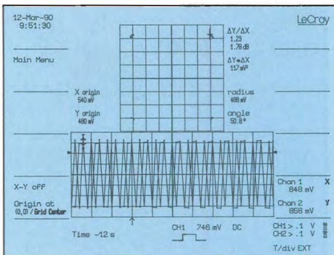
Figure 4. The same constellation diagram of a PSK signal as in Figure 3, with the crosshair cursor used to measure the [h]jitter.
