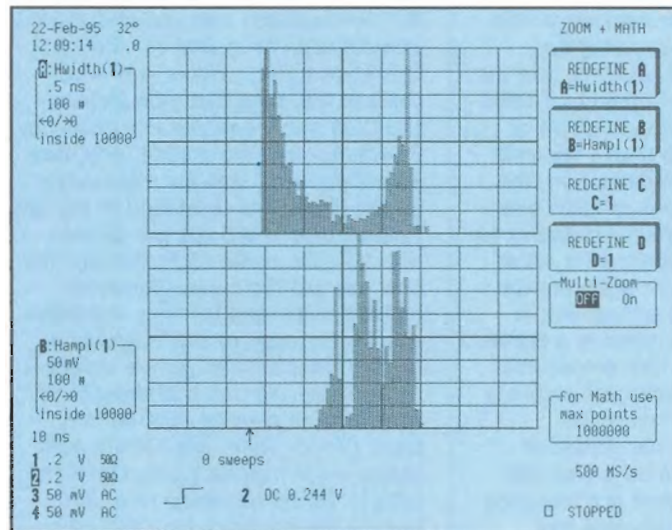
Figure 5: This figure shows an analysis of the widths (upper part of screen) and amplitude (lower half of the screen) of the bits in a data stream. Up to four histograms can be displayed simultaneously.
