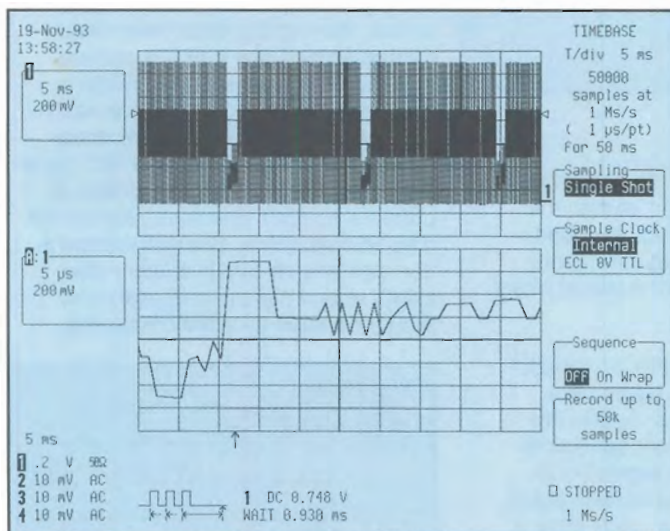
Figure 1: The 9354L always shows the maximum record length on screen, and sampling is always optimal. Note that the original trace and its expansion can be displayed simultaneously.
