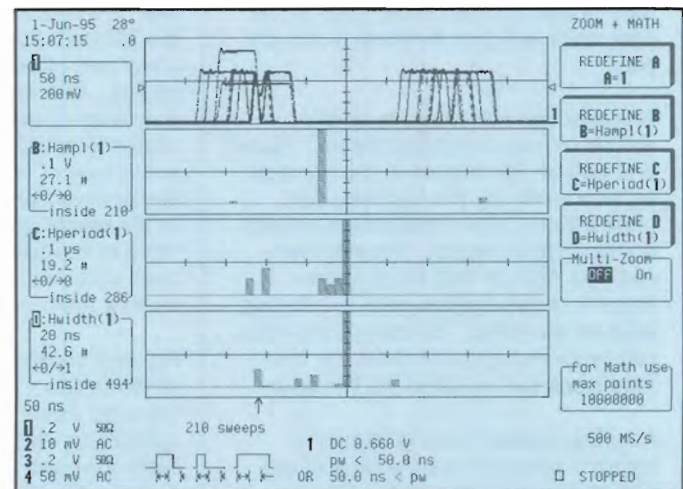
Figure 8. Bar chart showing histograms of the amplitude, period and width of events caught by the exclusion trigger.
