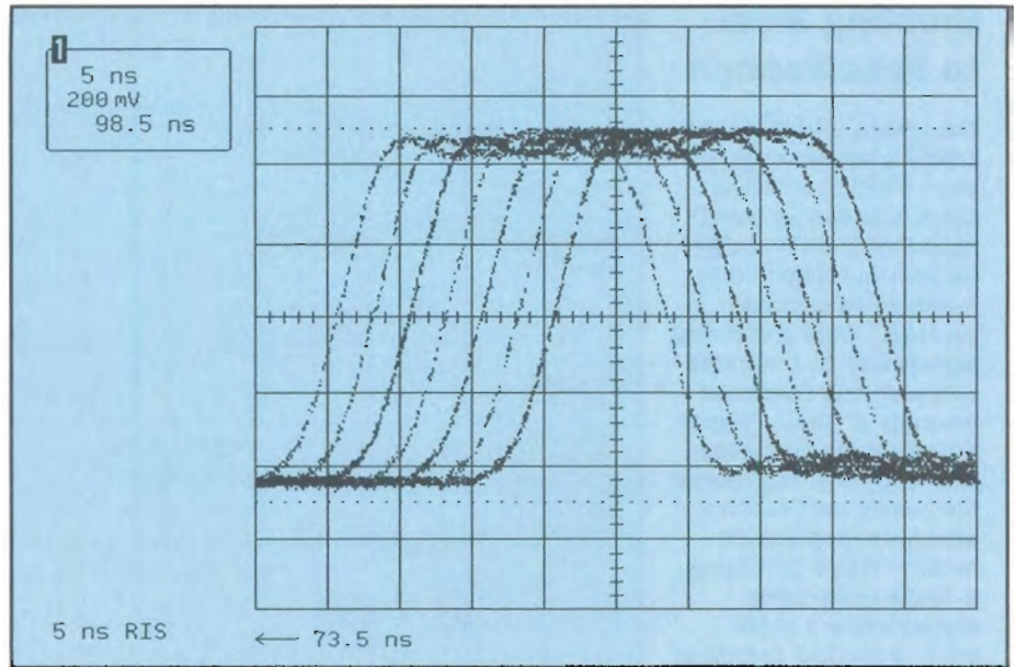
Figure 24. Persistence display showing jitter range
