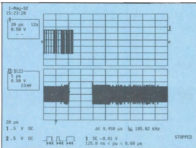
Figure 13. Capture of collisions on an Ethernet bus.
