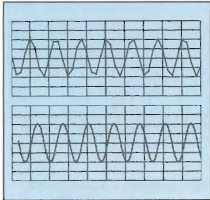
Sine wave digitized at 5 and 25 samples/cycle respectively, with straight line interpolation applied
