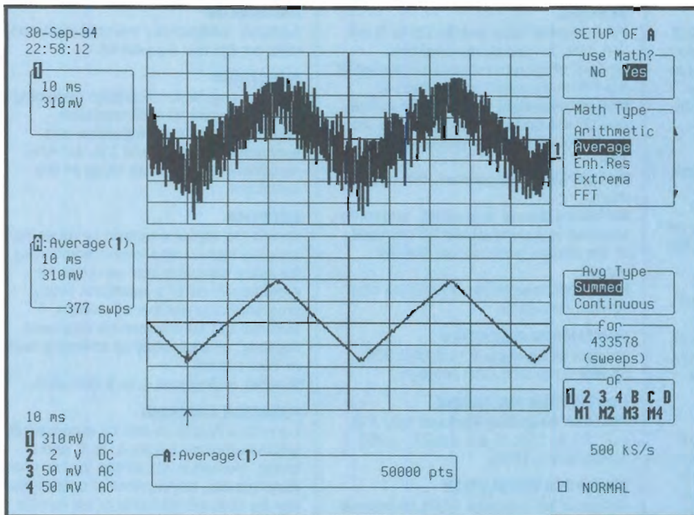
Summed Averaging is applied to the signal in Channel 1, to remove random noise. Trace A shows the result after 377 sweeps: the noise has practically disappeared.
