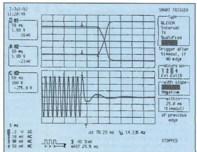
Figure 2: Measurement of the hold-up time. LeCroy's "Dropout" trigger mode is used, causing the scope to trigger on the mains drop which occur at the left of the lower trace.
