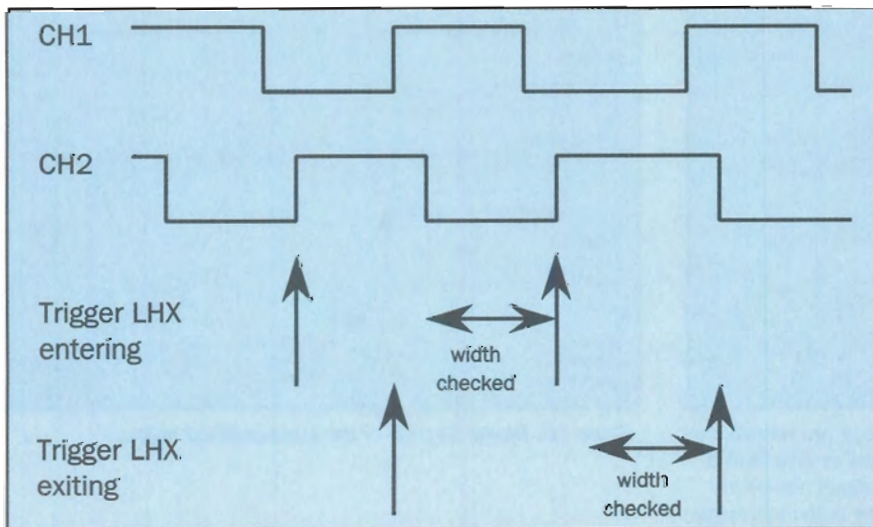
Figure 14: Timing diagram of the pattern trigger.
