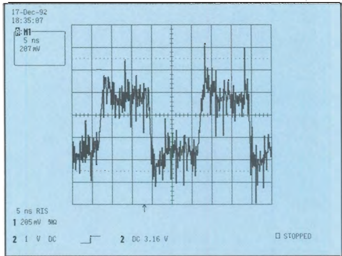
Figure 5. Noise removed by averaging.
