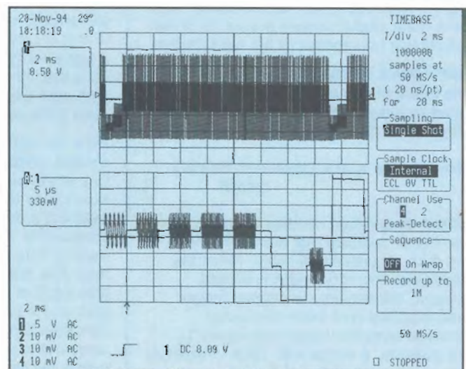
Figure 2b. Long memory enables a higher sampling rate: 1,000,000 samples captured. The zoom trace shows accurate details of the signal.
