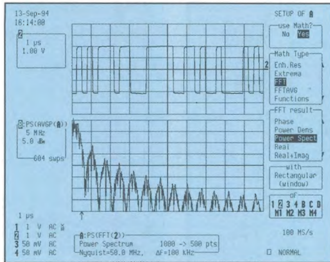
Figure 1: The top portion shows an AWG output of a spread spectrum communications signal which has been encoded by a "chipping" sequence. The lower portion shows a frequency analysis of the signal.
