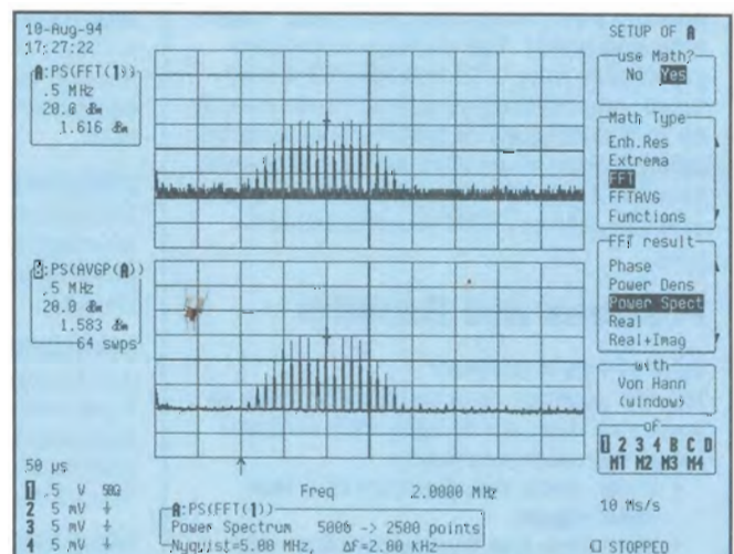
Frequency modulated signal, 2 MHz carrier with 99 kHz modulation frequency, 4:1 frequency deviation, FFT shows modulation sidebands, FFT power average used to improve s/n ratio.
